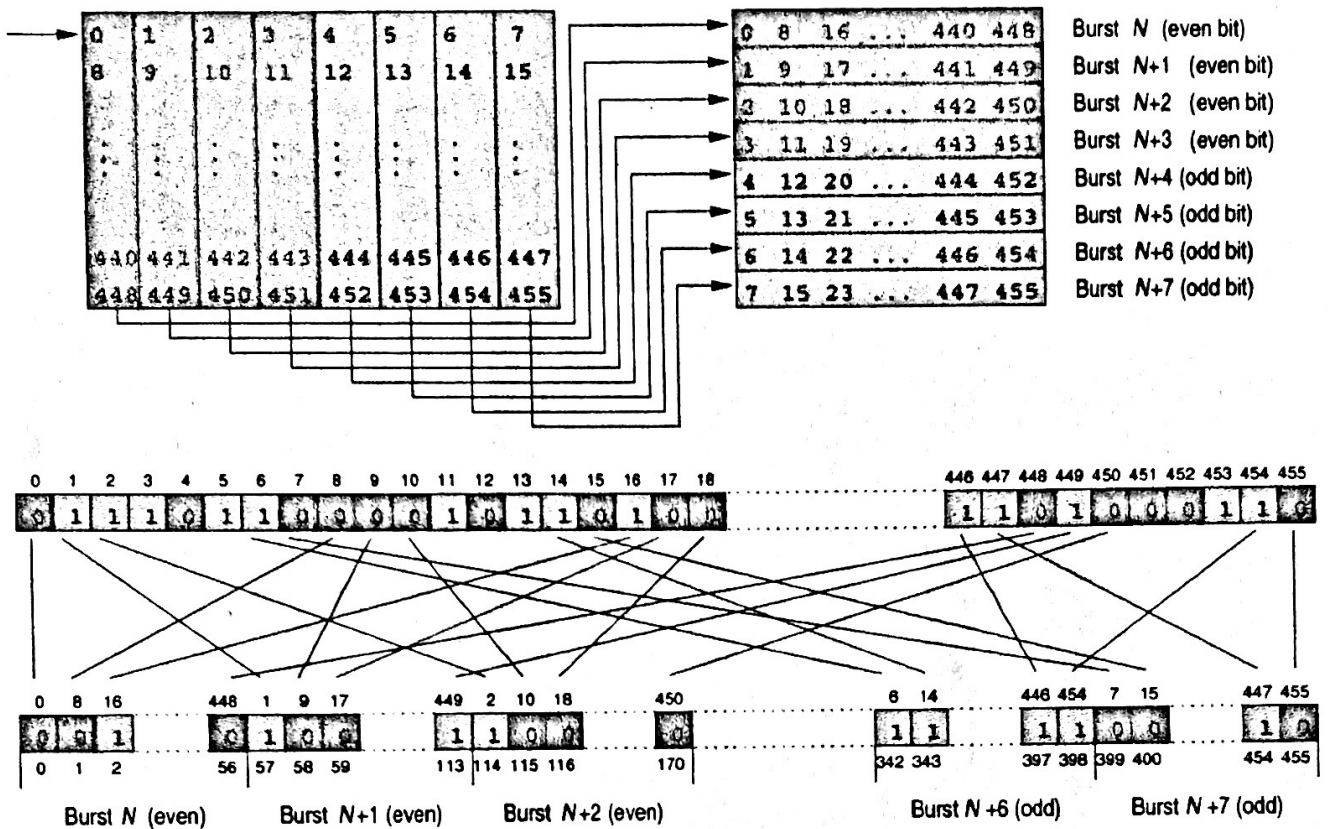
Figure 3.25: Example of interleaving
