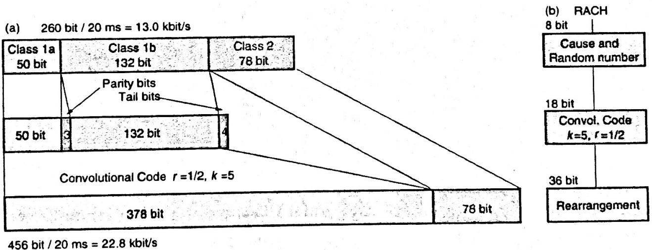
Figure 3.26: Channel coding for (a) speech transmission and (b) signalling
